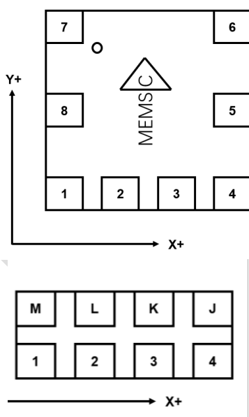
Figure 2: Sensing direction
