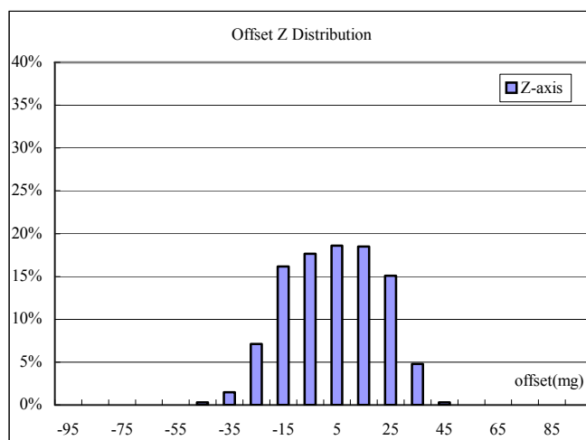
0g Z Offset Deviation
