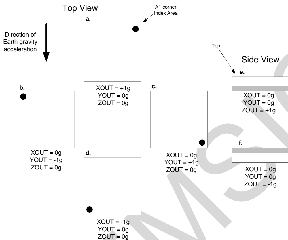
Figure 3. Package Orientation
