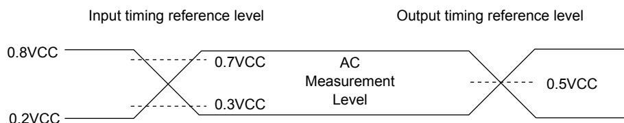
Figure 106. DATA INPUT TEST WAVEFORMS AND MEASUREMENT LEVEL
