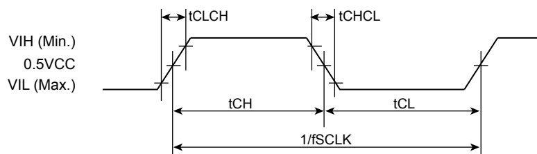
Figure 108. SCLK TIMING DEFINITION
