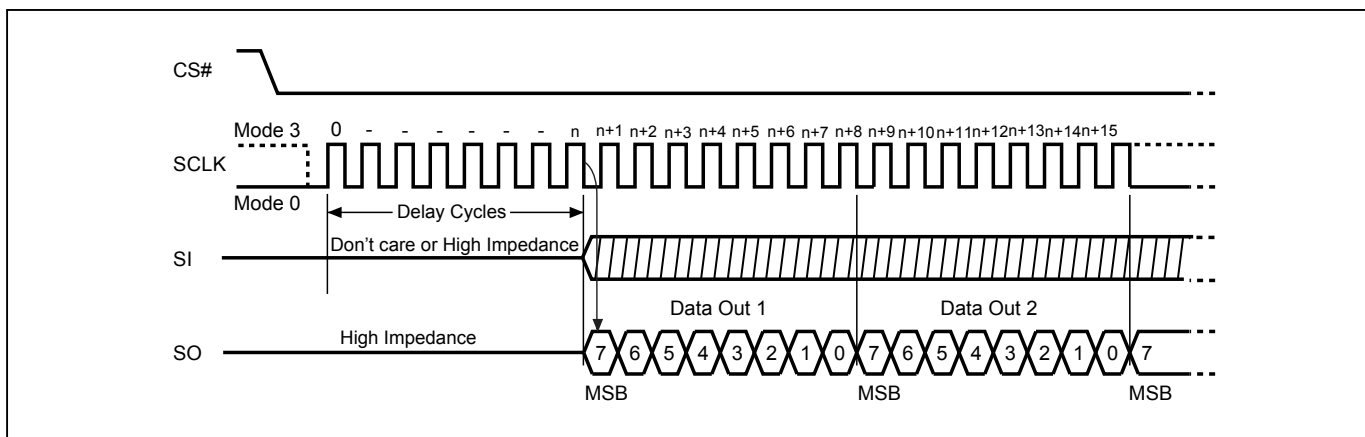
Figure 75. Fast Boot Sequence (QE=0)
