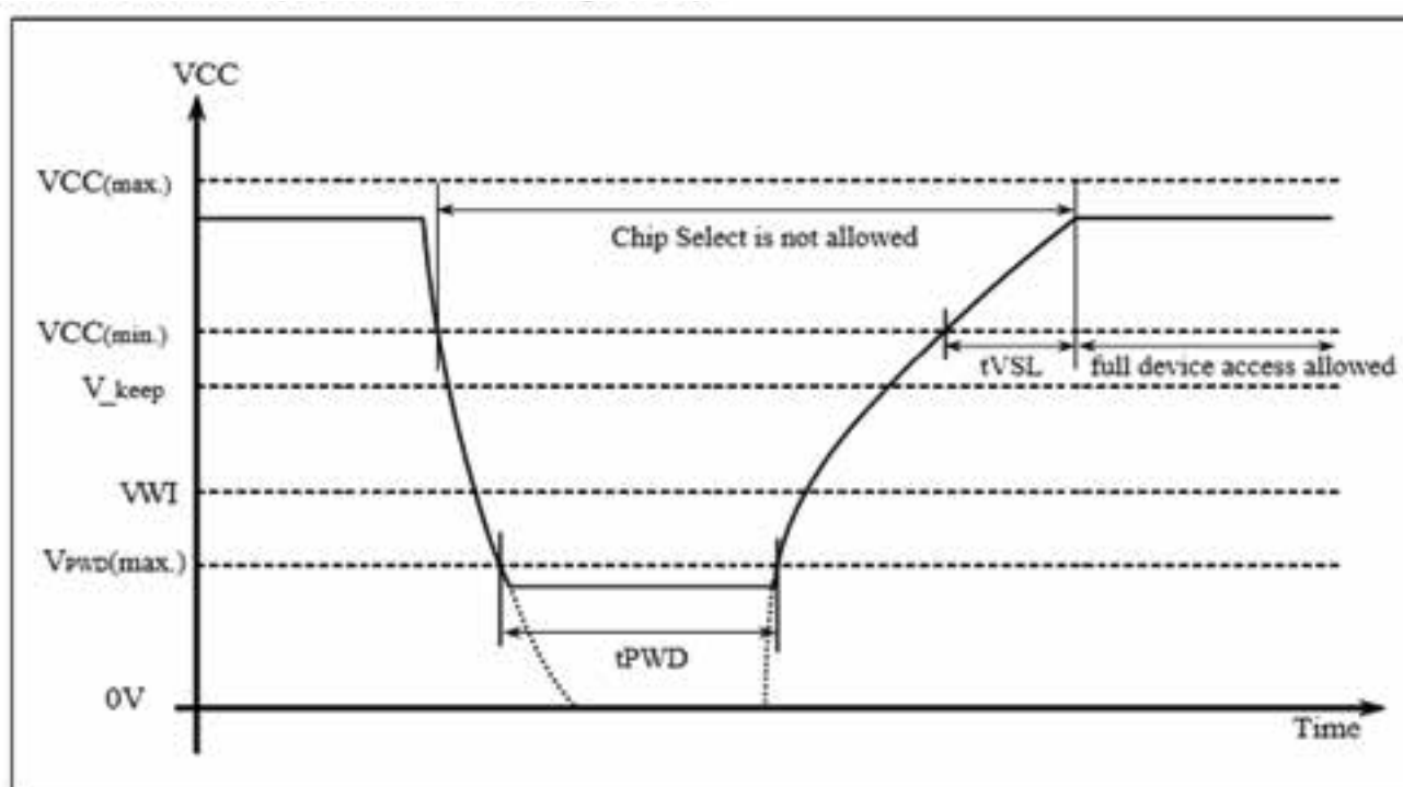
Figure 35. Power Up/Down and Voltage Drop
