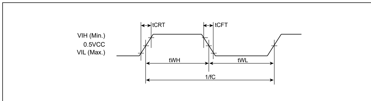
Figure 38. SCLK TIMING DEFINITION
