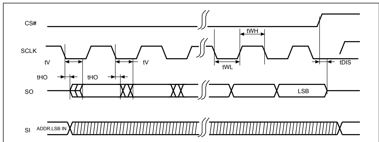
Figure 41. Serial Output Timing
