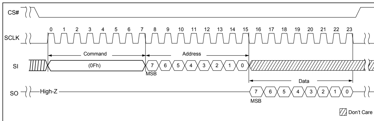
Figure 7. GET FEATURE (0Fh) Timing
