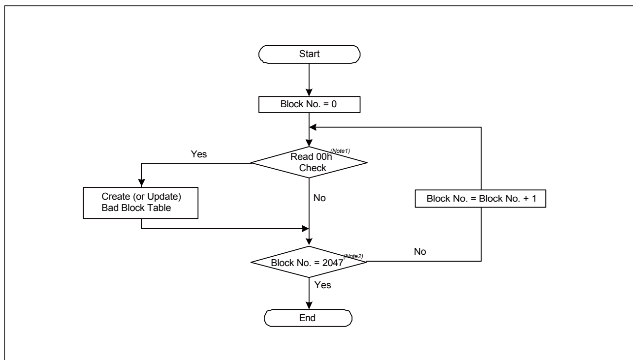
Figure 36. Bad Block Test Flow
