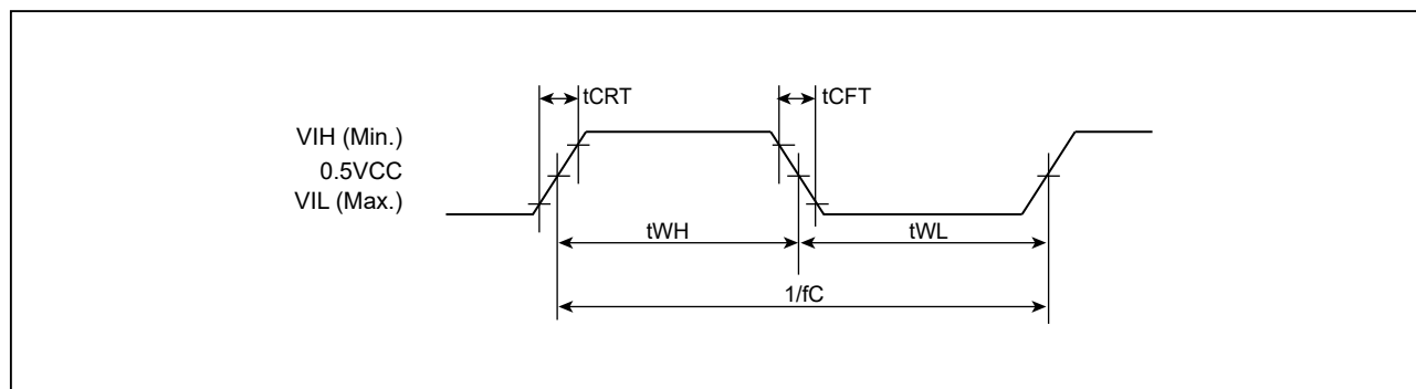
Figure 44. SCLK TIMING DEFINITION
