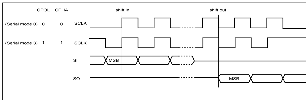
Figure 4. Serial Mode Supported
