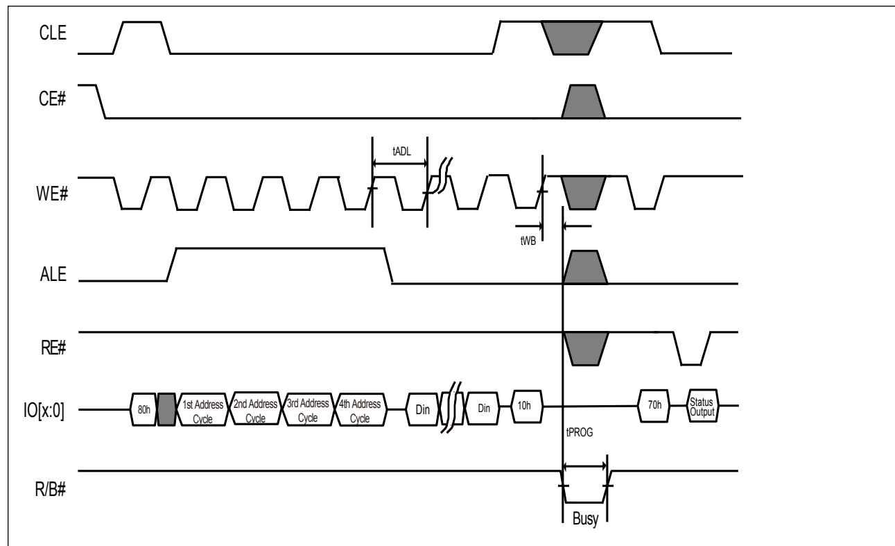
Figure 30. AC Waveforms for OTP Data Program
