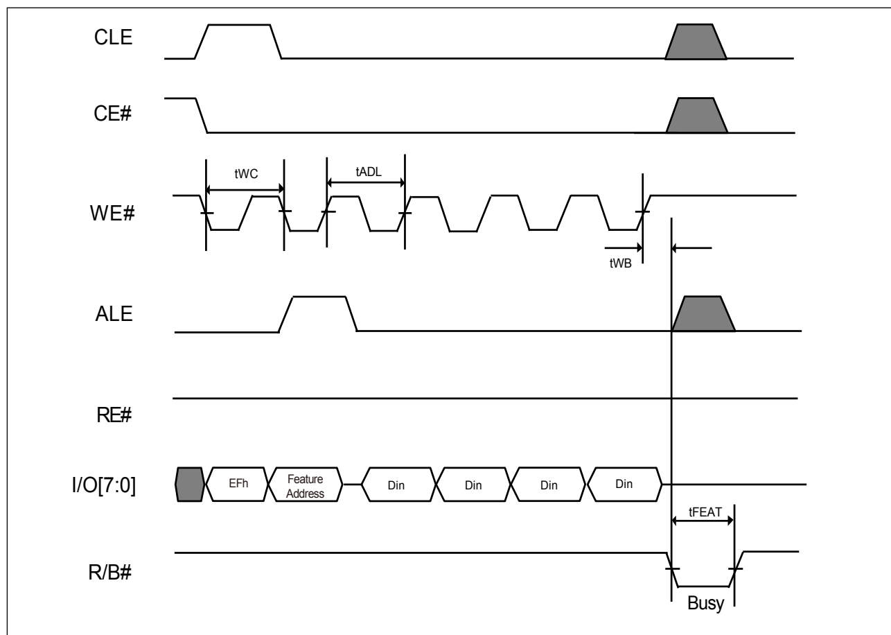
Figure 28-1. AC Waveforms for Set Feature (ONFI) Operation
