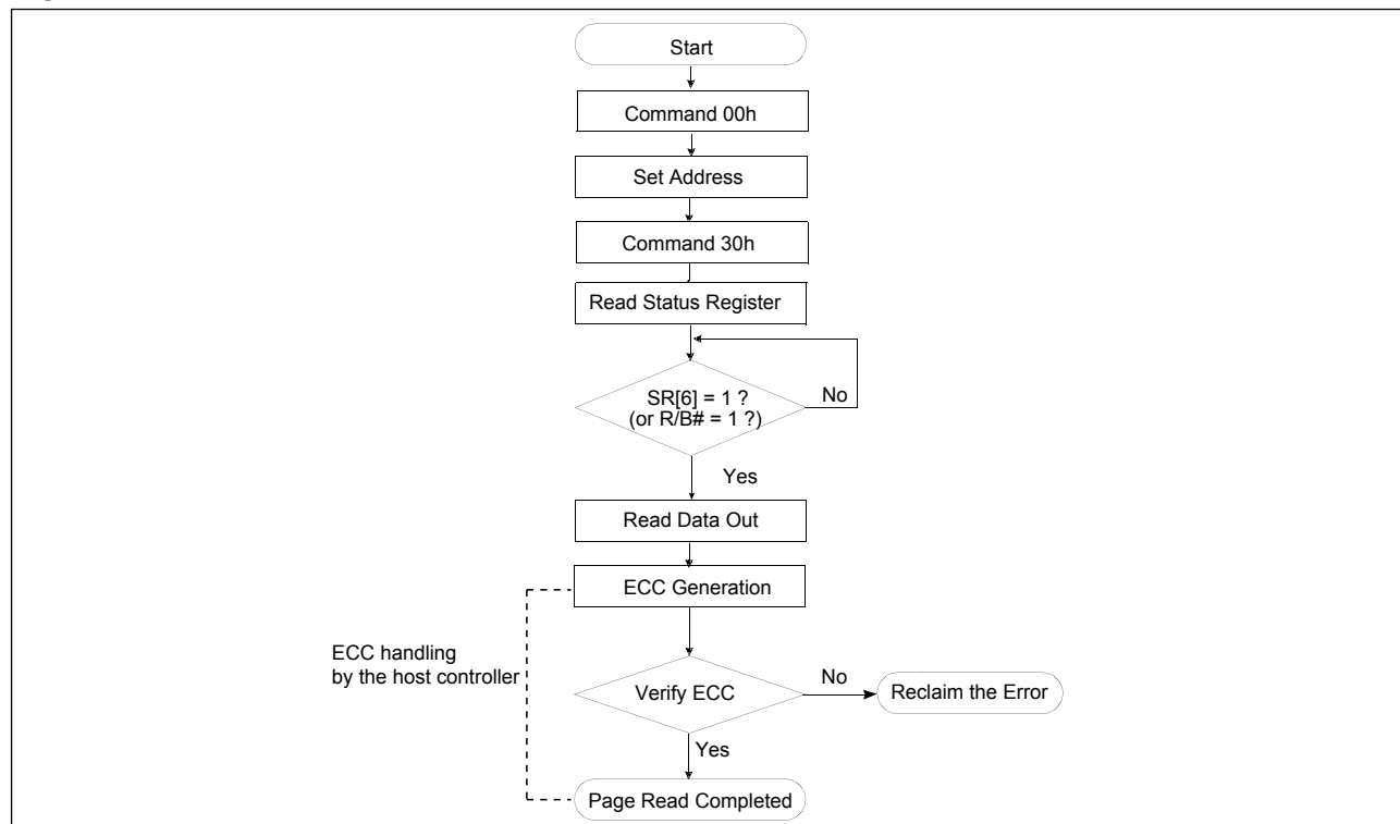
Figure 53. Read Flow Chart
