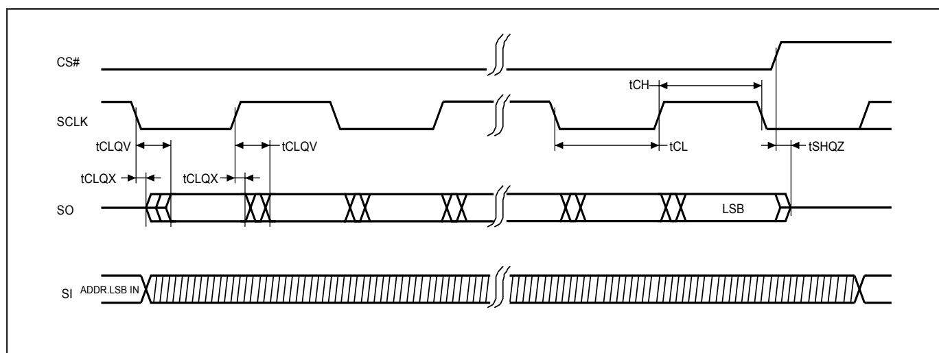
Figure 5. Output Timing (DTR mode)
