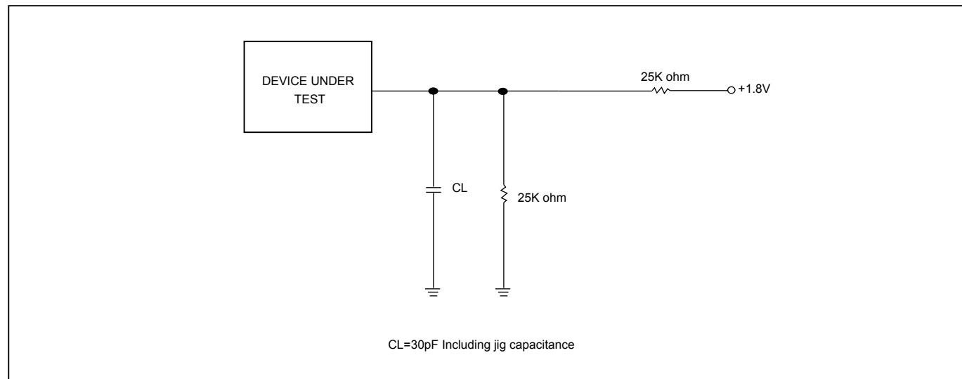
Figure 105. OUTPUT LOADING
