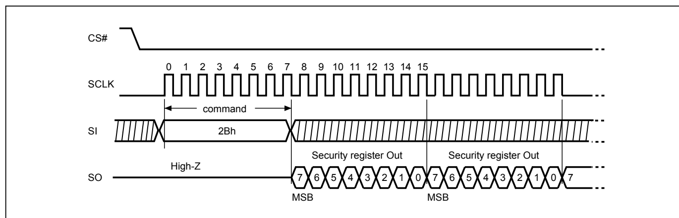
Figure 55. Read Security Register (RDSCUR) Sequence (SPI Mode)
