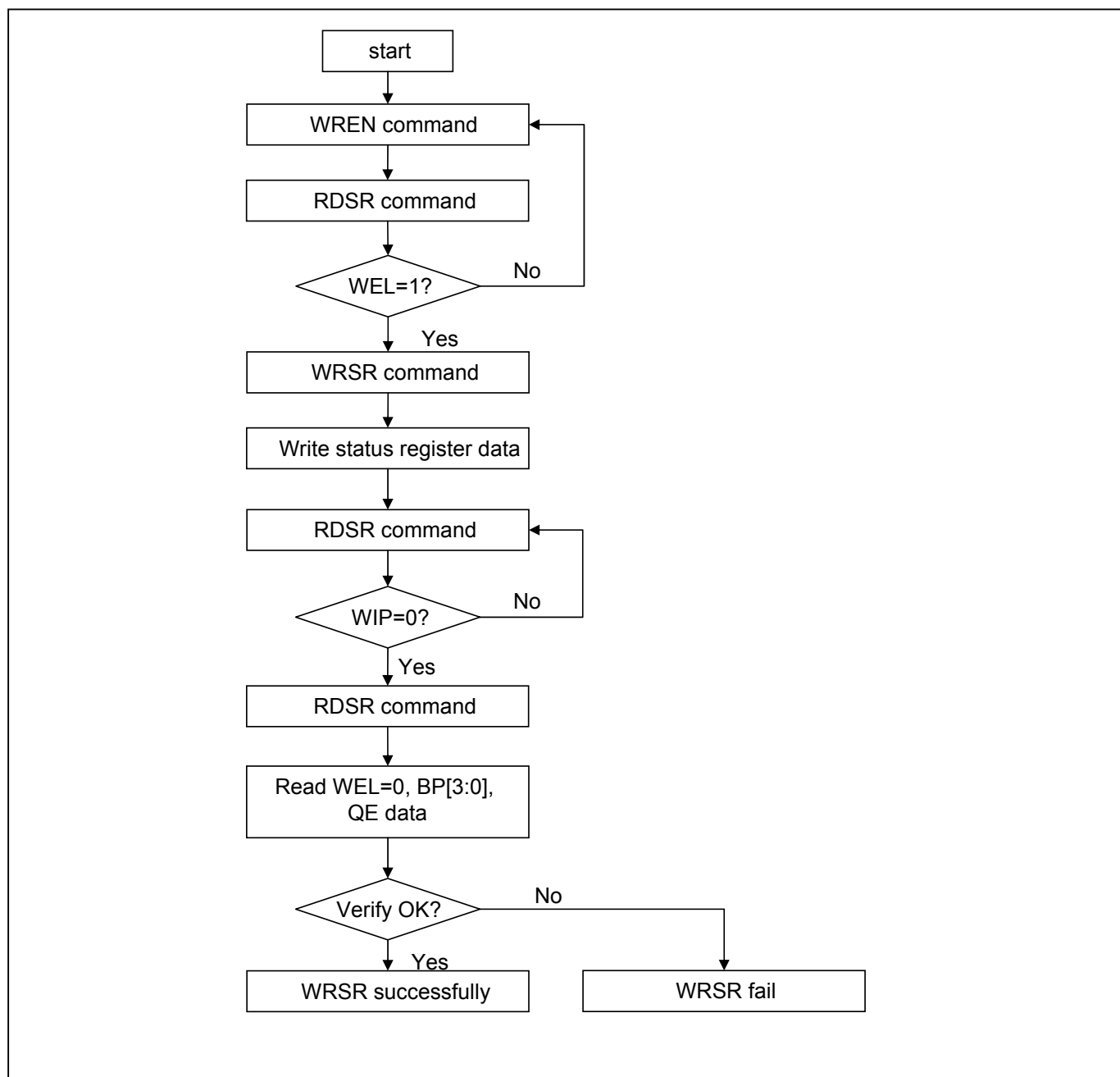
Figure 25. WRSR flow
