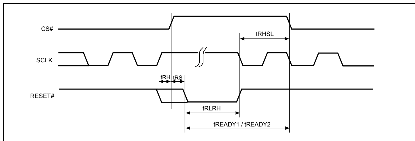
Figure 77. RESET Timing
