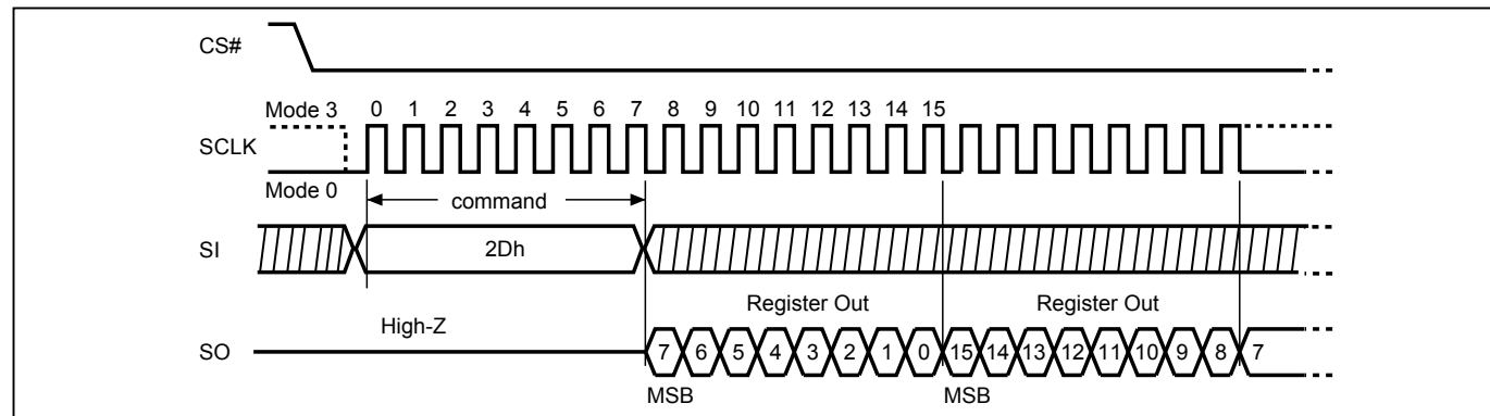
Figure 62. Read Lock Register (RDLR) Sequence (SPI Mode only)
