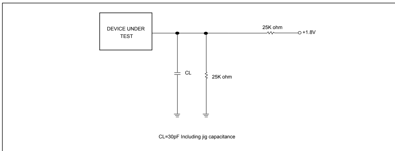
Figure 81. OUTPUT LOADING
