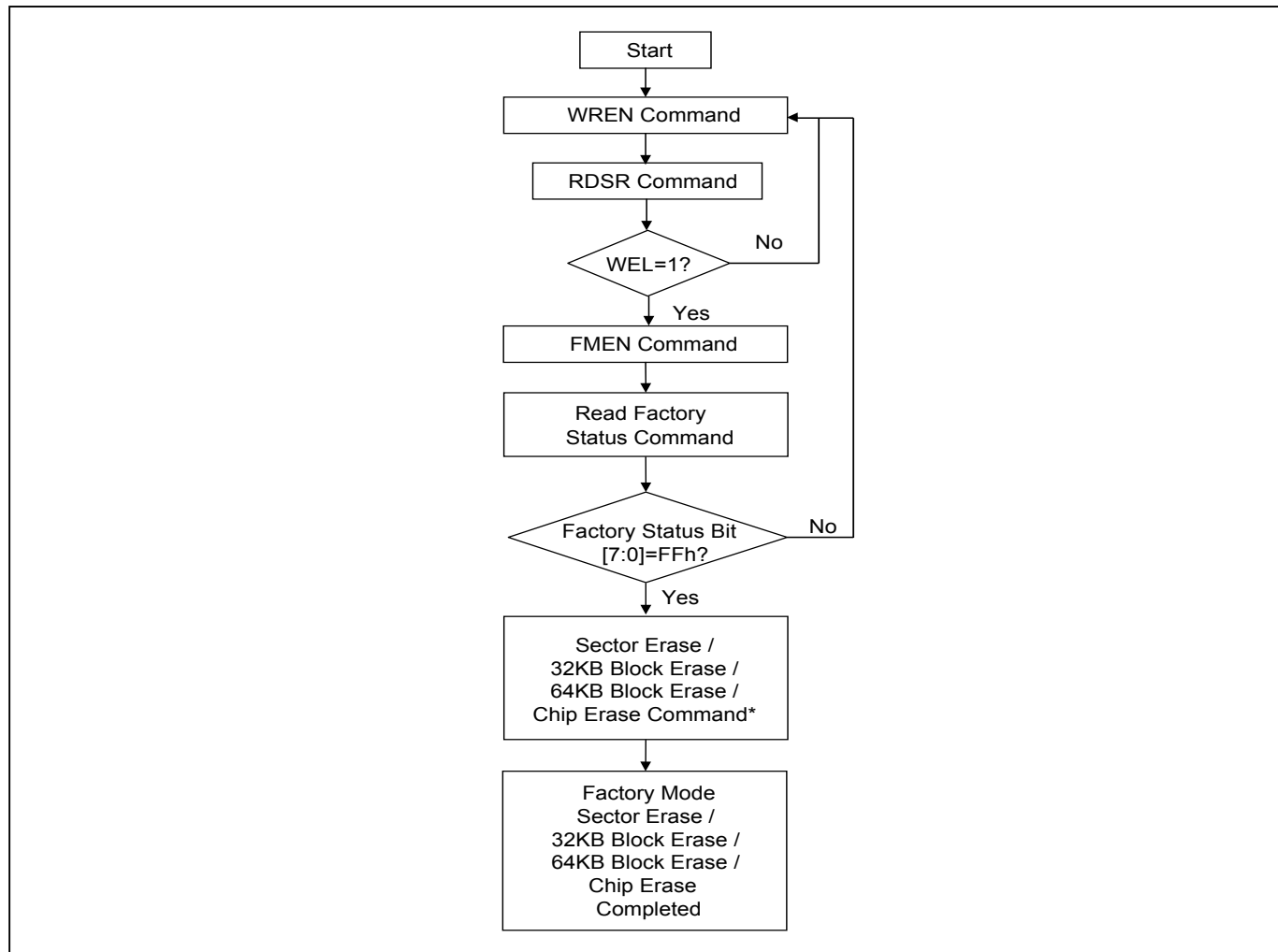
Figure 49. Factory Mode Erase Flow
