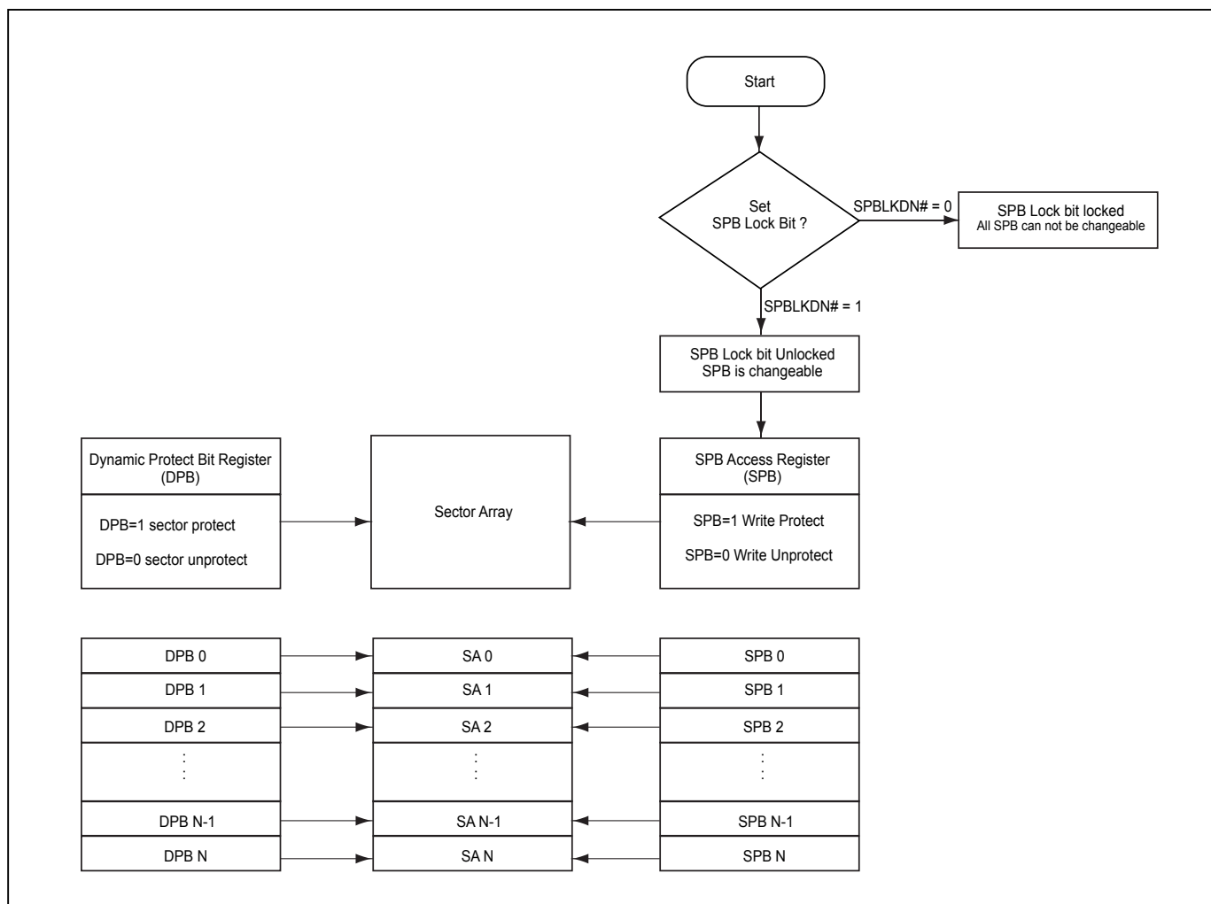
Figure 61. Advanced Sector Protection Overview
