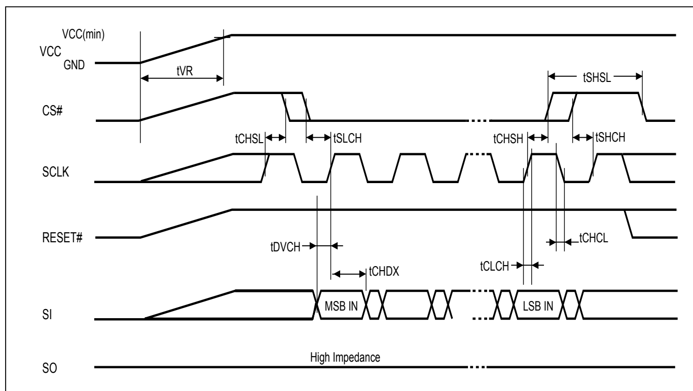
Figure 83. AC Timing at Device Power-Up
