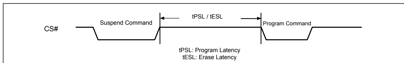
Figure 70. Suspend to Program Latency
