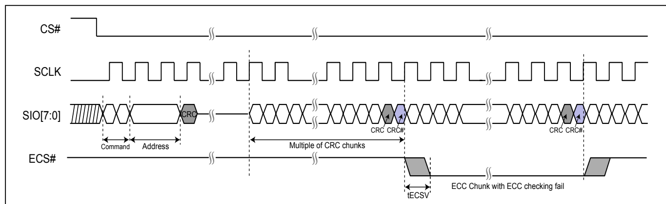
Figure 119. CRC Timing (With CRC# output)
