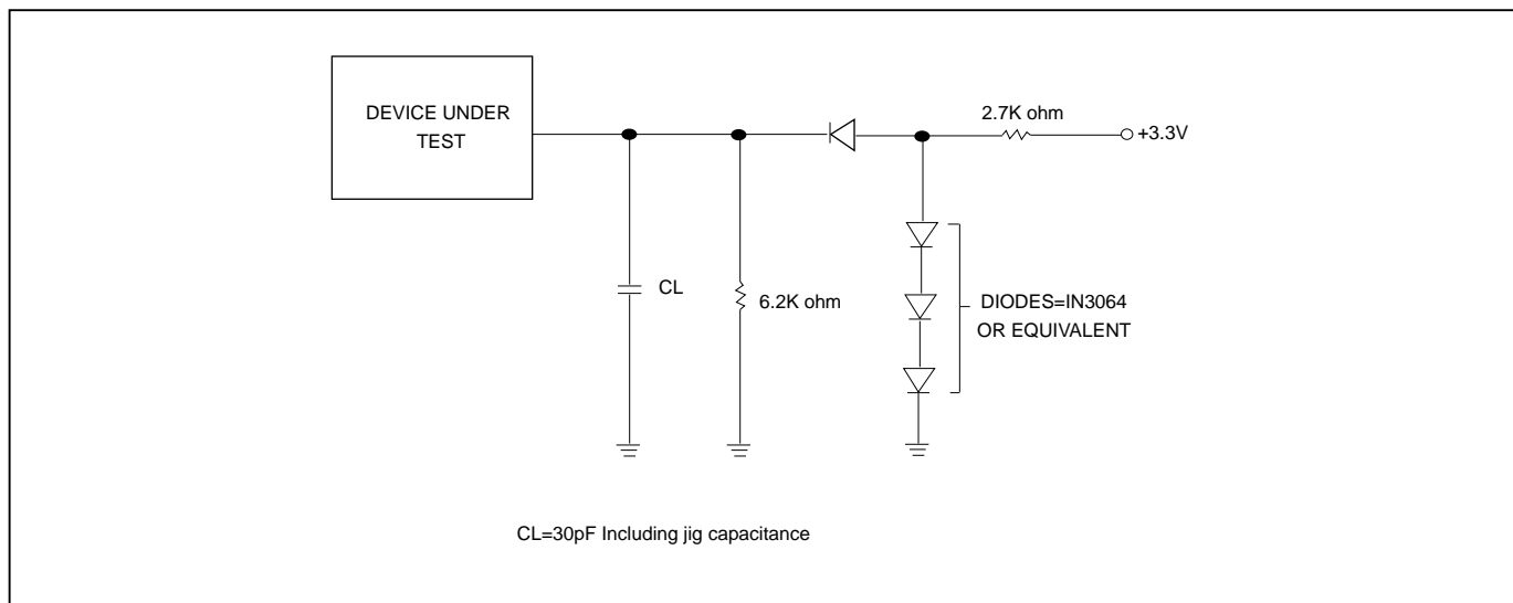
Figure 5. OUTPUT LOADING
