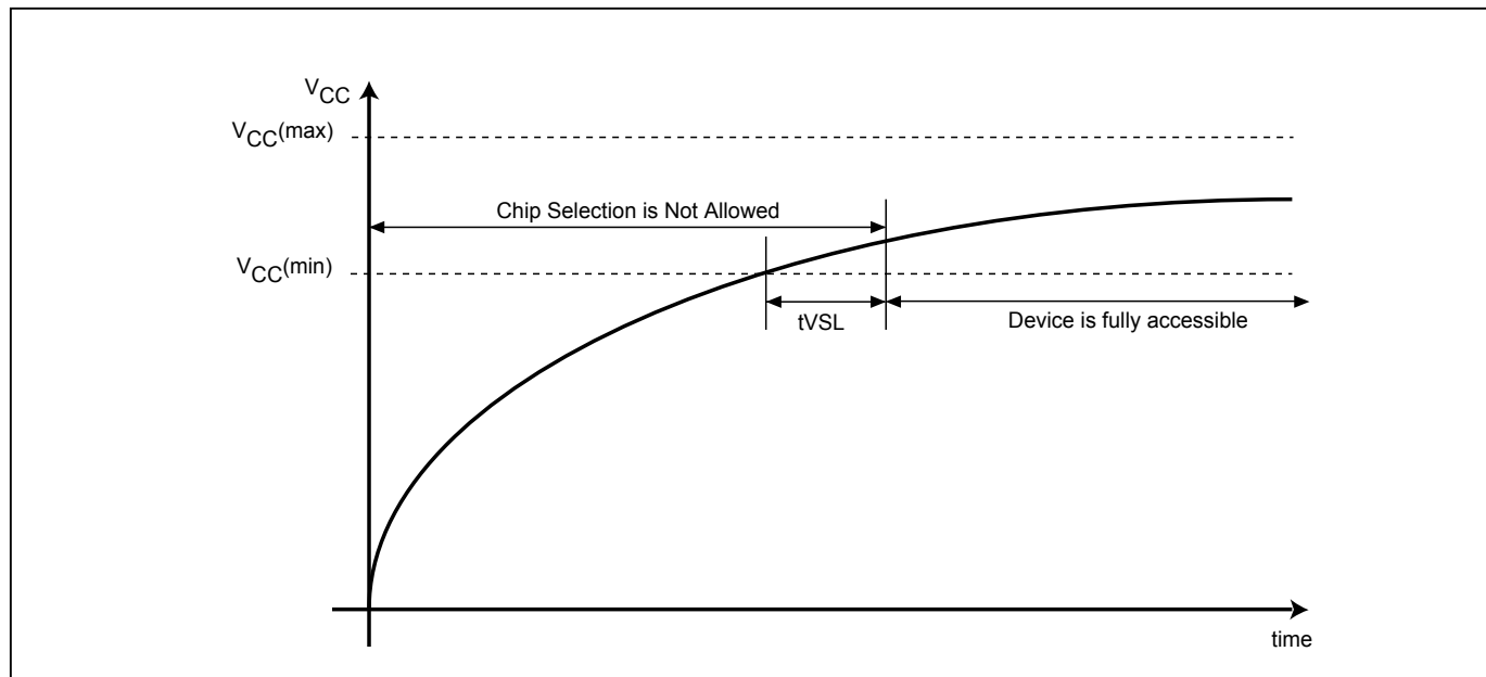
Figure 28. Power-up Timing
