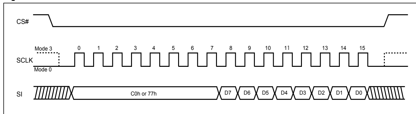
Figure 17. Burst Read
