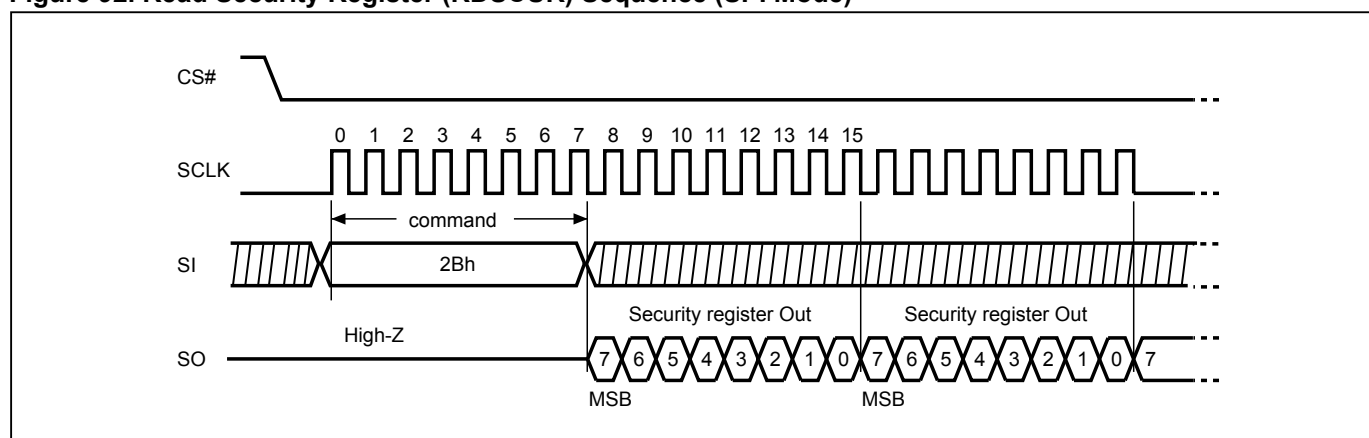
Figure 92. Read Security Register (RDSCUR) Sequence (SPI Mode)
