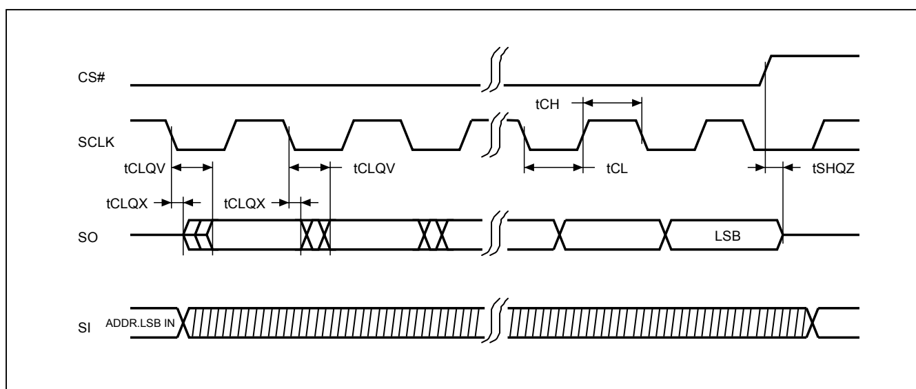
Figure 41. Output Timing
