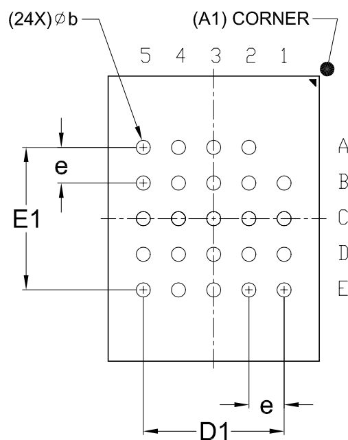
BOTTOM VIEW
