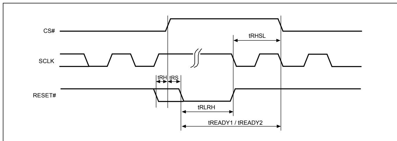
Figure 78. RESET Timing
