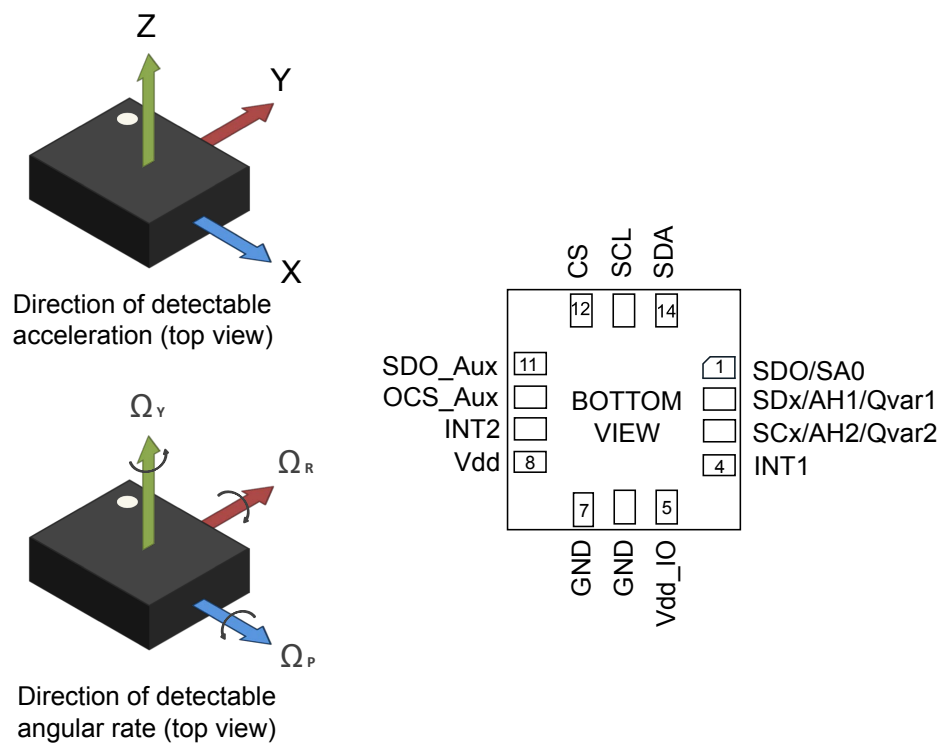
Figure 5. Pin connections
