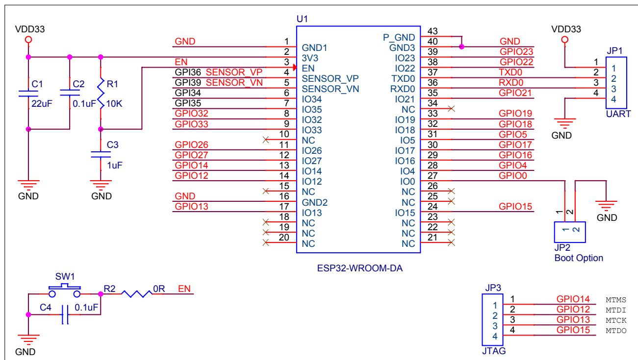
Figure 5: Peripheral Schematics
