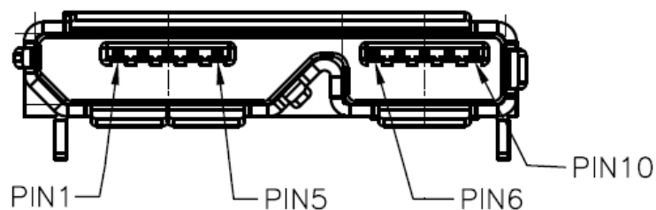
Figure 2. USB 3.0 Micro B Type Connector Drawing
