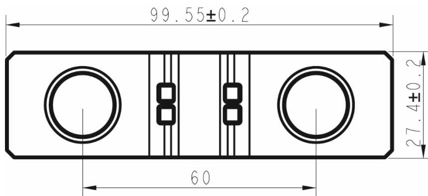
Figure 5. eAP87606D100 Side View
