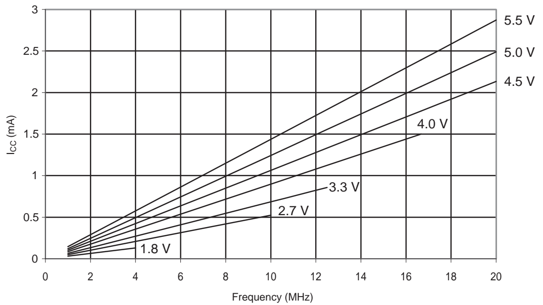
Figure 29-183. ATmega328P: Reset Supply Current vs. Frequency (1 - 20 MHz)
