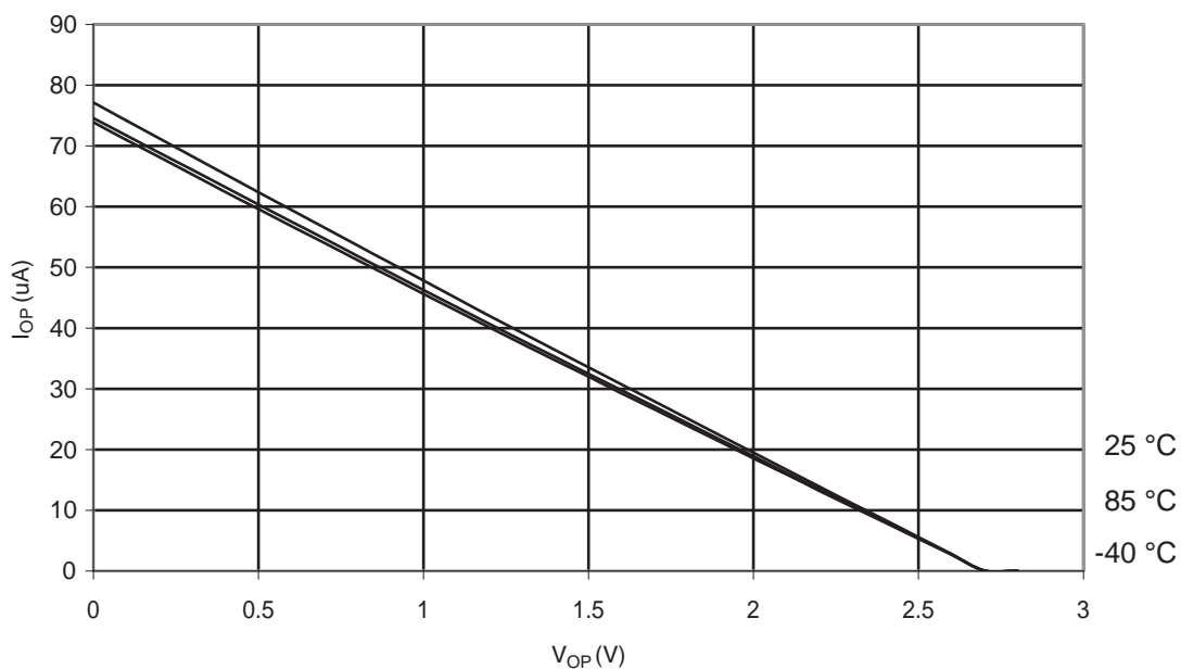
Figure 29-154. ATmega328P: I/O Pin Pull-up Resistor Current vs. Input Voltage ( V_{CC} = 2.7\text{ V} )
