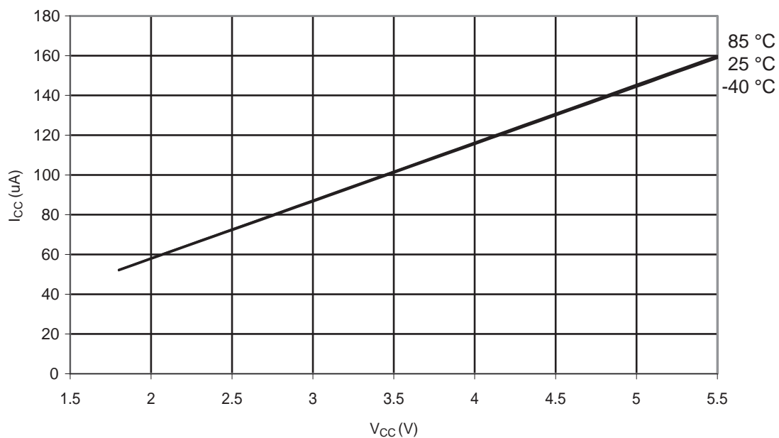
Figure 29-179. ATmega328P: AREF External Reference Current vs. V_{CC}
