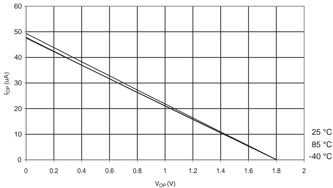
Figure 29-153. ATmega328P: I/O Pin Pull-up Resistor Current vs. Input Voltage ( V_{CC} = 1.8\text{ V} )
