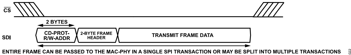
Figure 20. MAC Frame: Transmit
