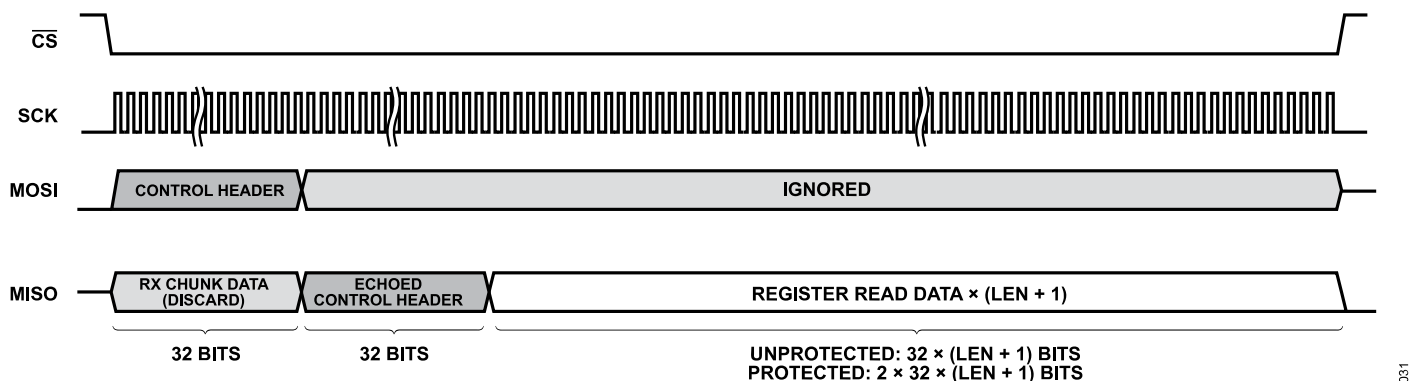
Figure 28. Control Read Transaction
