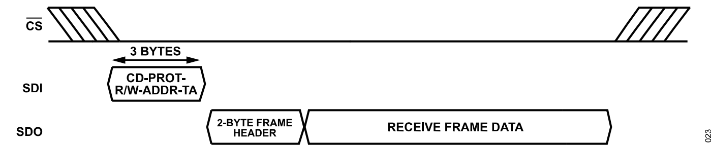
Figure 21. MAC Frame: Receive
