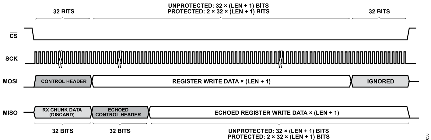
Figure 27. OPEN Alliance Control Transaction
