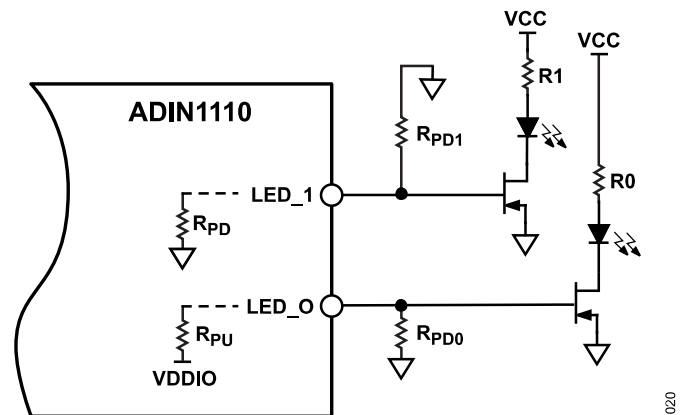
Figure 17. Recommended Transistor Controlled LED Circuit
