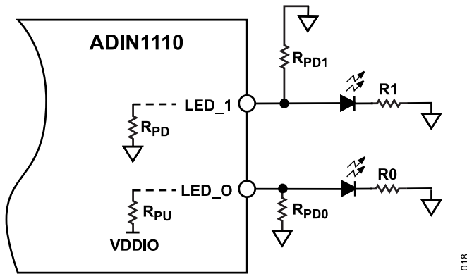
Figure 15. Recommended Active High LED Circuit
