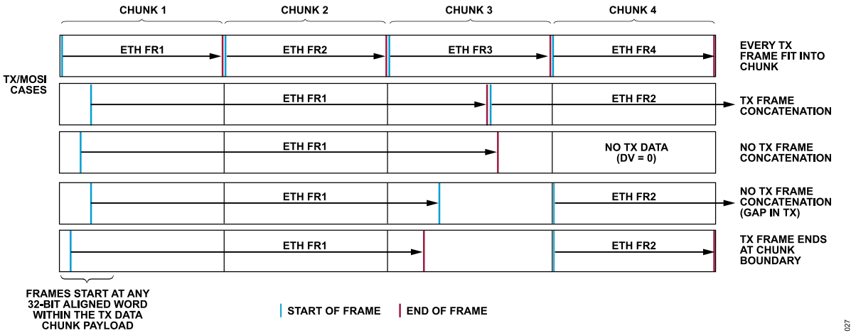
Figure 25. Transmit Data Chunk Cases
