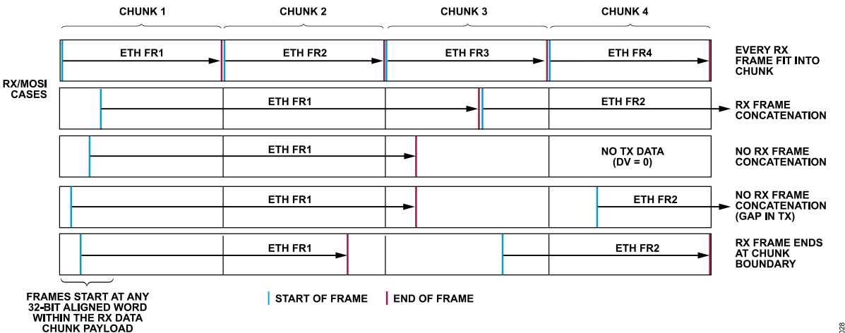
Figure 26. Receive Data Chunk Cases
