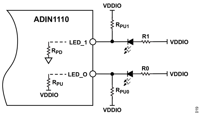
Figure 16. Recommended Active Low LED Circuit
