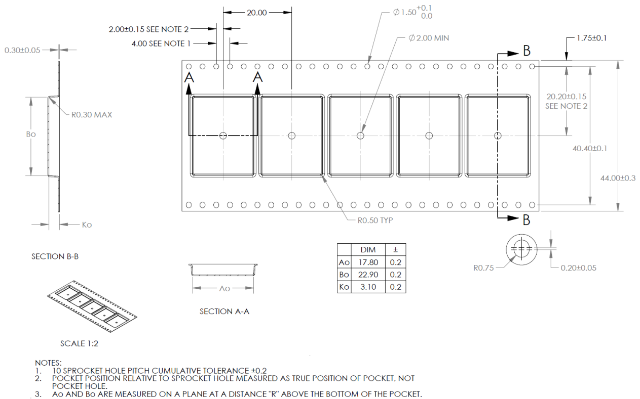
Figure 54: ZED-F9P tape dimensions (mm)
