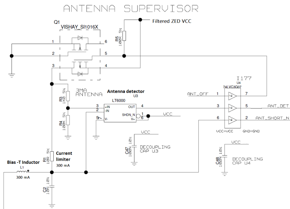
Figure 24: ZED-F9P antenna supervisor
