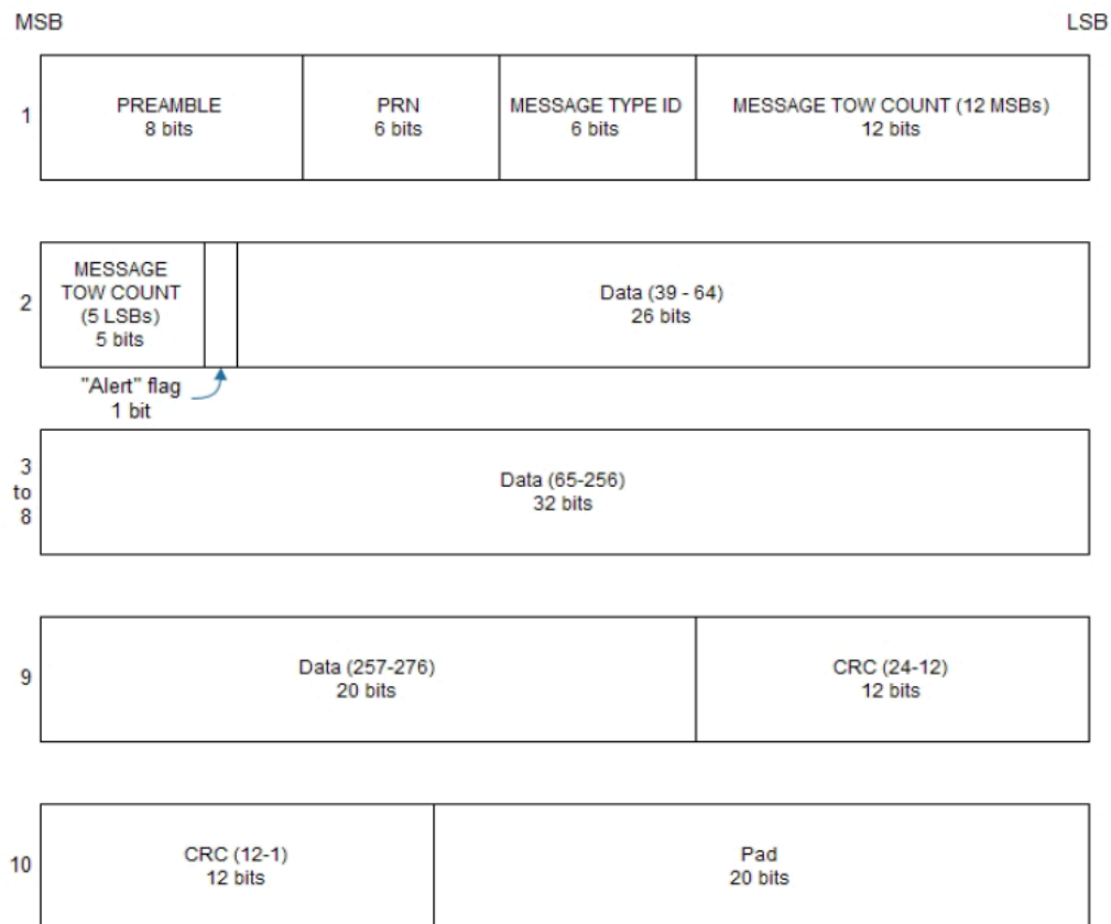
Figure 30: GPS L2C subframe words
