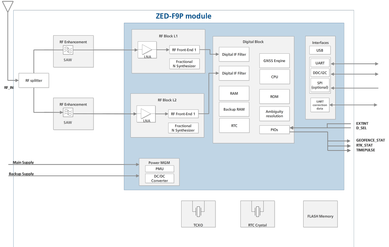
Figure 1: ZED-F9P block diagram
