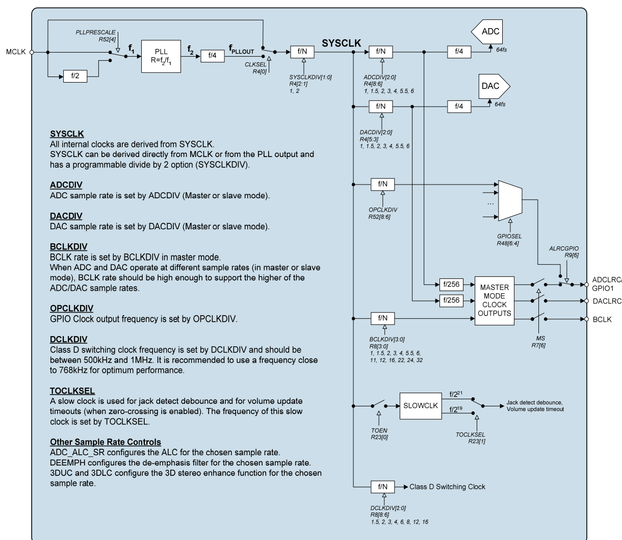
Figure 36 Clocking Scheme
