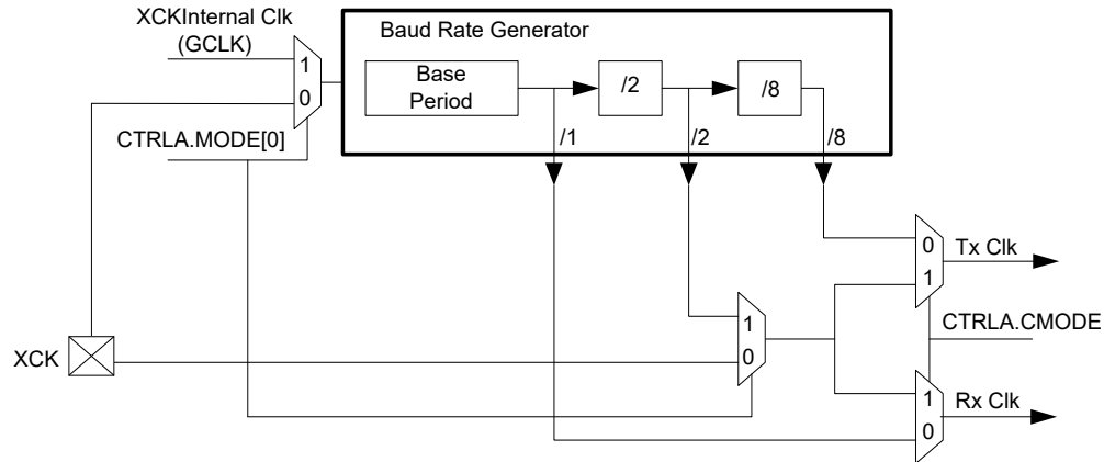
Figure 26-3. Clock Generation
