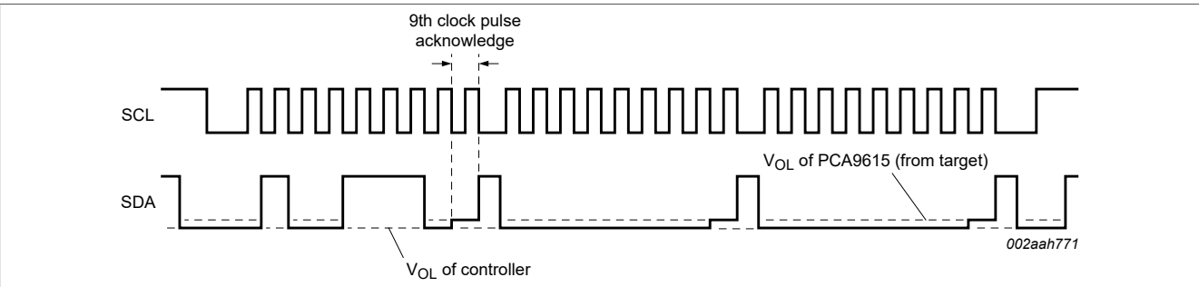
Figure 12. Single-ended bus waveform (controller side of bus)
