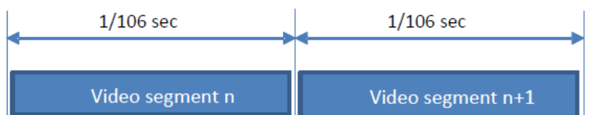
Figure 39 - Clock Too Slow - Failure to Read an Entire Frame Within the Frame Period
