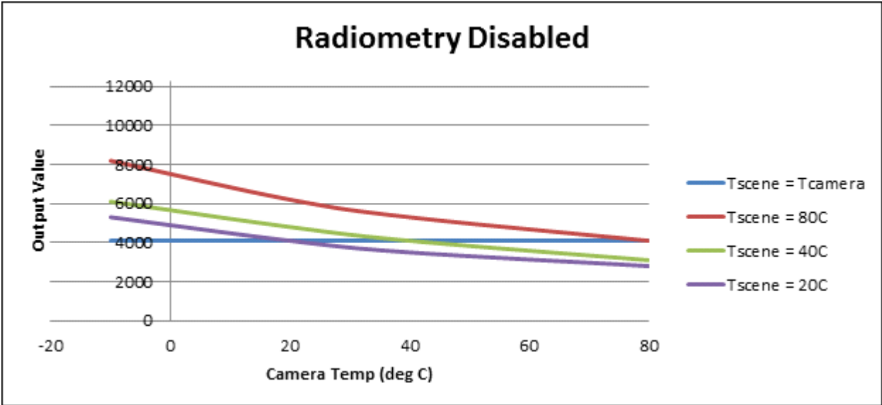
Figure 11 - Hypothetical Illustration of Camera Output vs. Camera Temperature in Radiometry-disabled Mode
