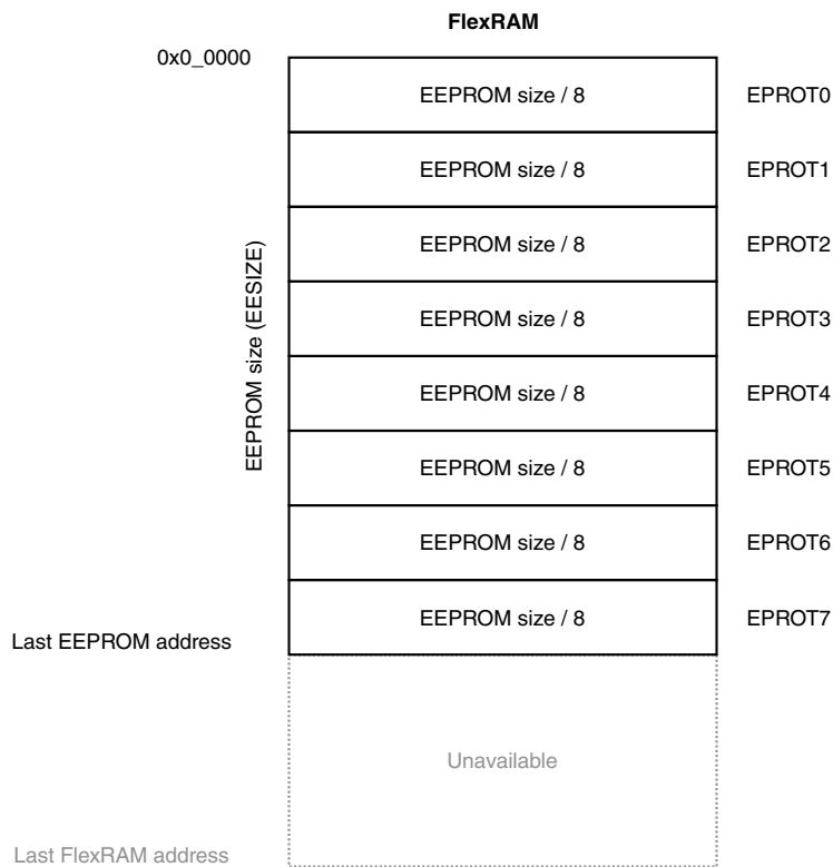
Figure 32-8. EEPROM protection
