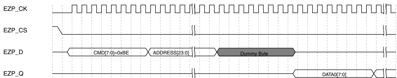
Figure 33-15. Read FlexRAM at High Speed command sequence
