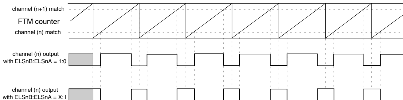
Figure 40-228. Combine mode
