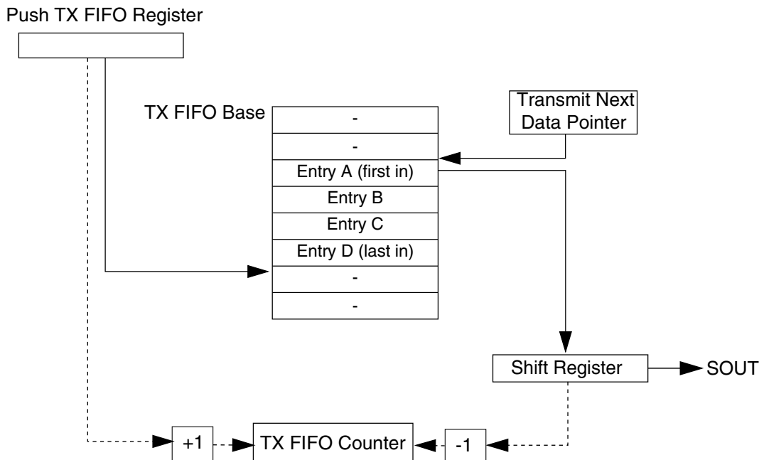
Figure 50-100. TX FIFO pointers and counter
