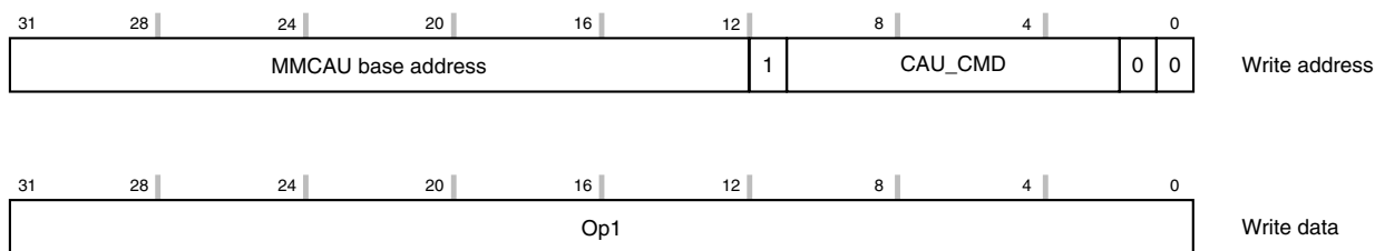
Figure 33-14. Indirect loads
