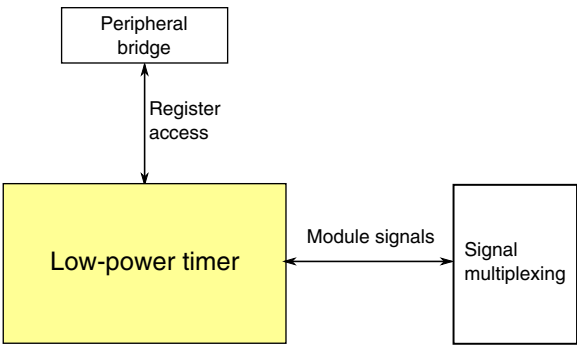
Figure 3-46. LPTMR configuration
