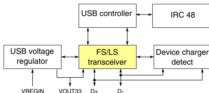
Figure 3-51. USB FS/LS Subsystem Overview
