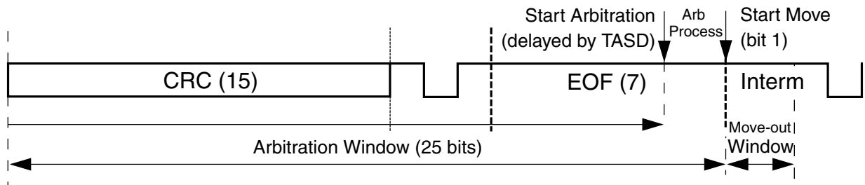
Figure 49-69. Arbitration and move-out time windows
