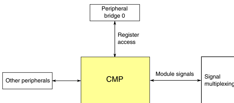
Figure 3-38. CMP configuration
