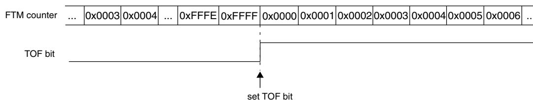
Figure 40-213. Example when the FTM counter is free running
