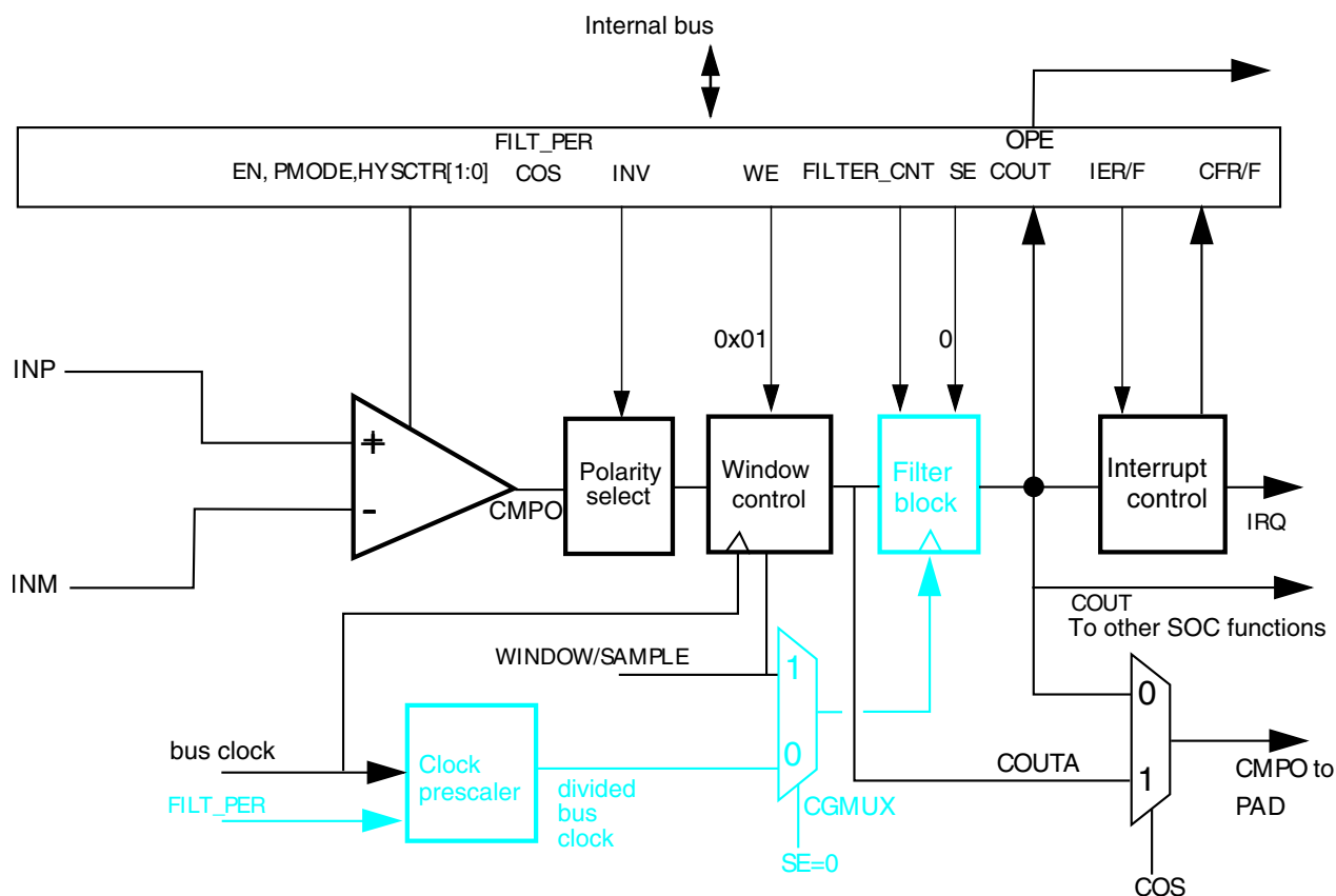
Figure 36-33. Windowed mode
