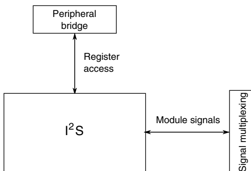
Figure 3-63. I²S configuration
