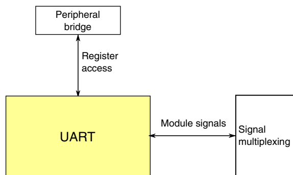
Figure 3-61. UART configuration
