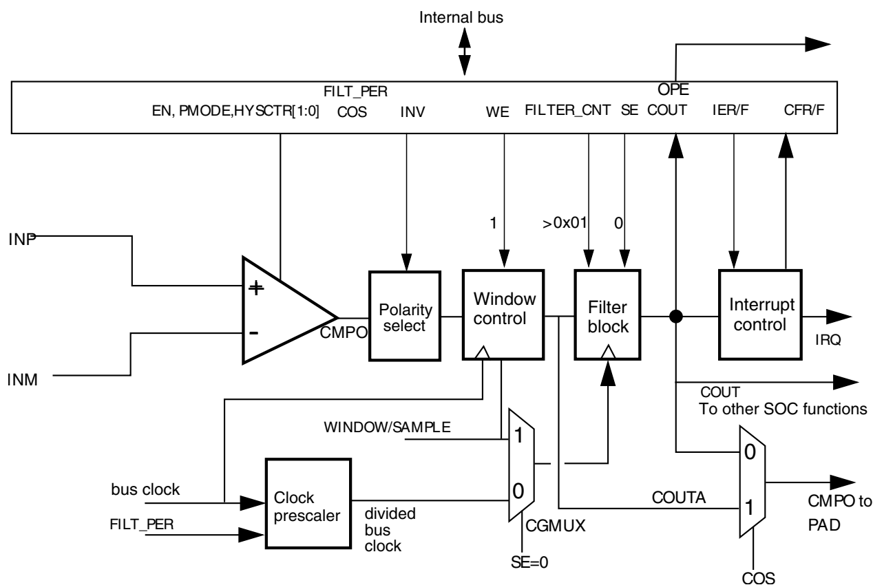
Figure 36-35. Windowed/Filtered mode
