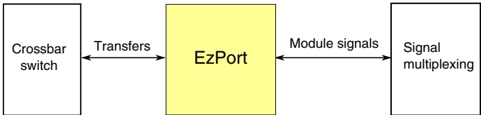
Figure 3-29. EzPort configuration
