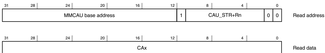
Figure 33-15. Indirect store
