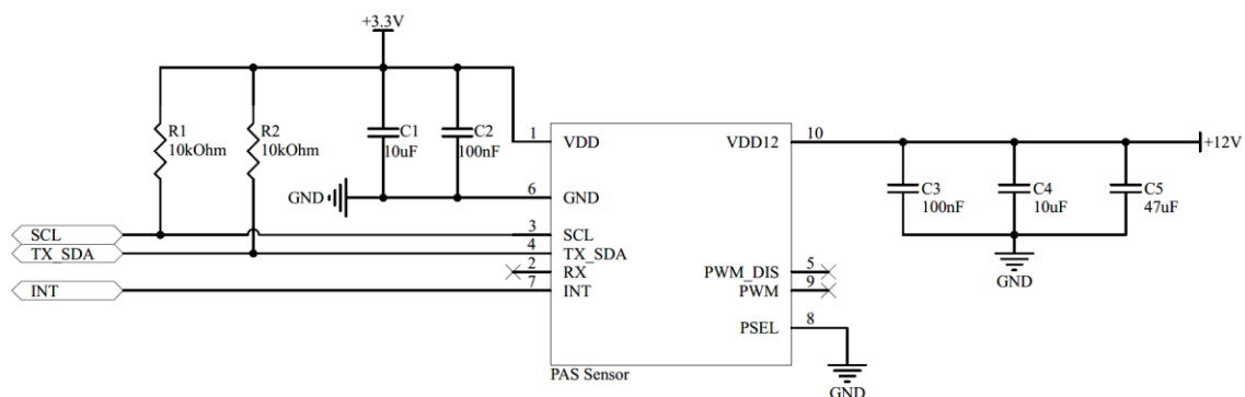
Figure 6 Application circuit example for I2C
