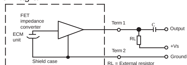
Schematic Diagram:
