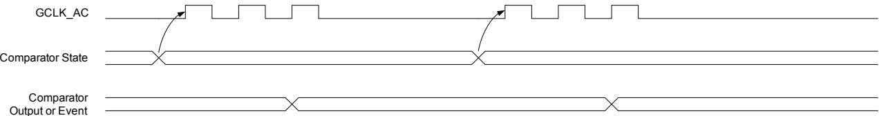
Figure 33-9. Continuous Mode SleepWalking
