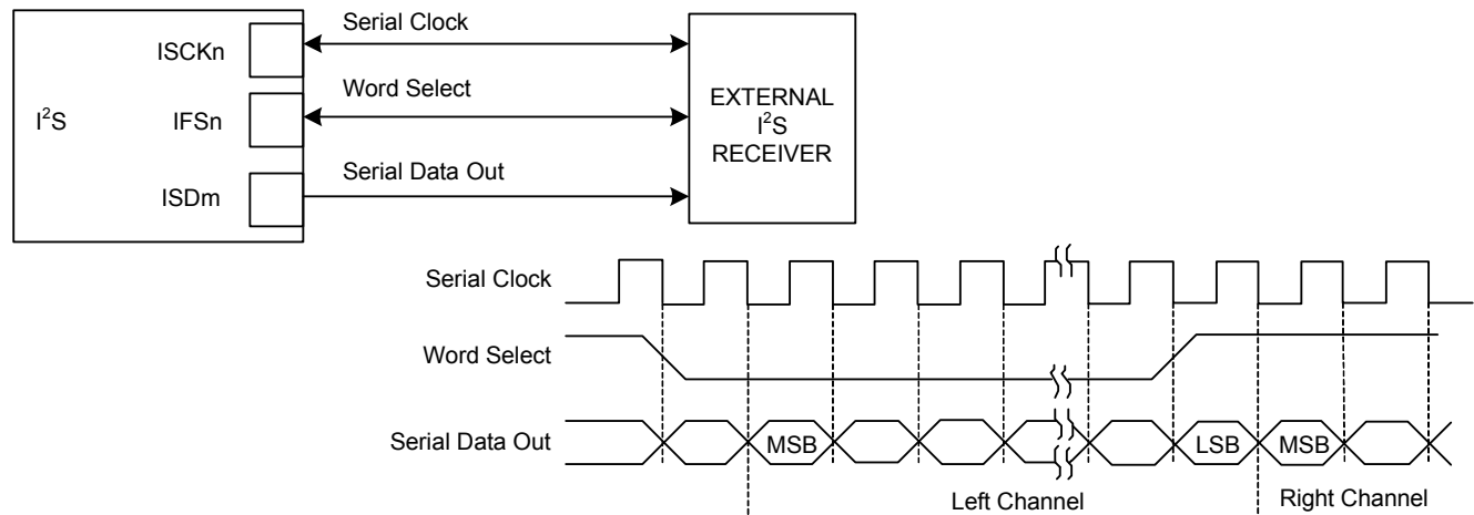
Figure 28-7. Audio Application Block Diagram
