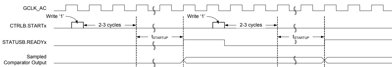
Figure 33-3. Single-Shot Example
