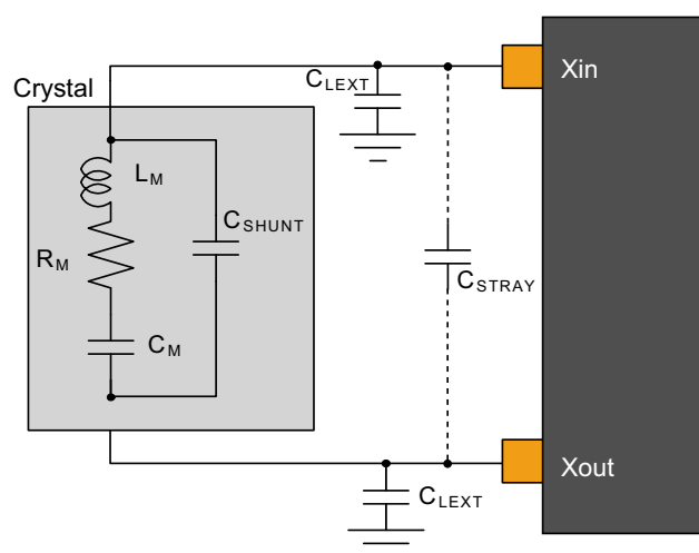
Figure 36-6. Oscillator Connection
