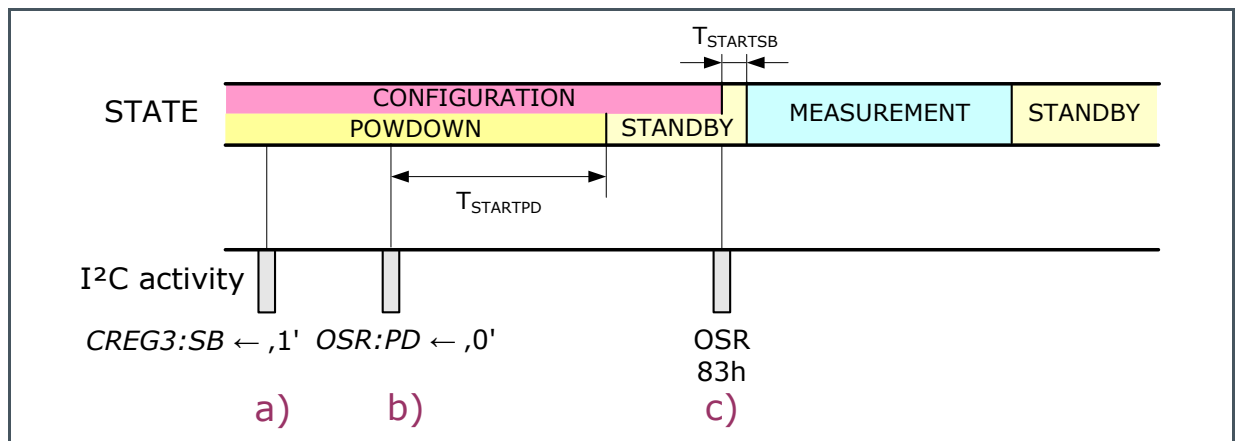
Figure 20: Principle Start and Stop Sequence of a Measurement After Startup with \text{OSR:PD} = "0" and \text{CREG3:SB} = "1"
