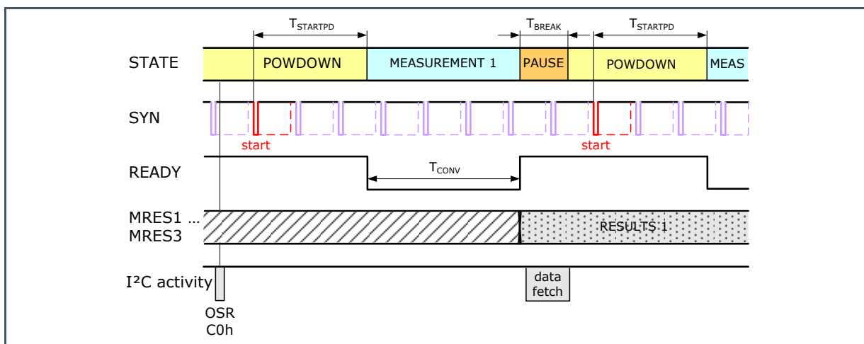
Figure 25: Principle Sequence of Measurement in SYNS Mode ( OSR:PD , OSR:SS are set to "1")
