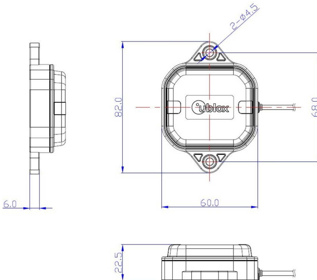
Figure 1: ANN-MB series mechanical drawing. Dimensions are given in mm.
