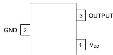
SC59
