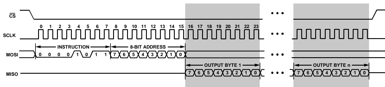
Figure 38. Burst Read
