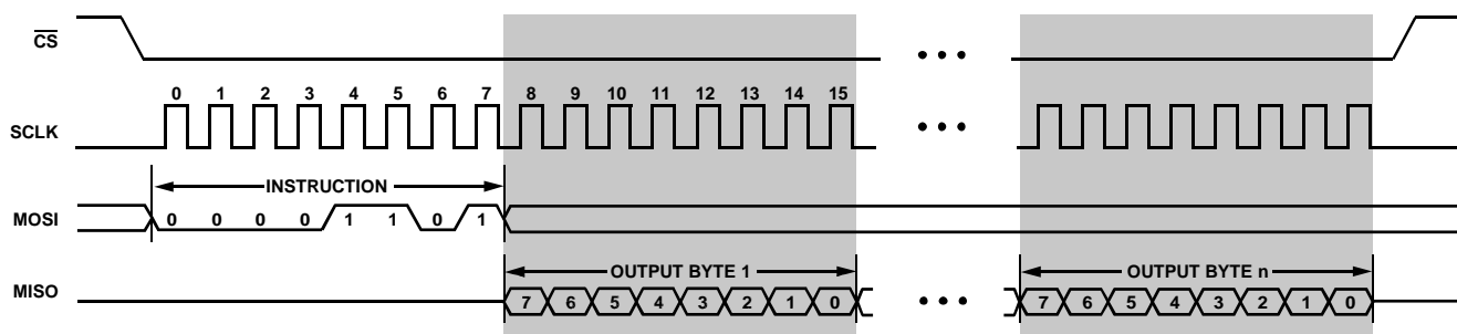
Figure 40. FIFO Read
