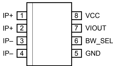
Pinout Diagram
