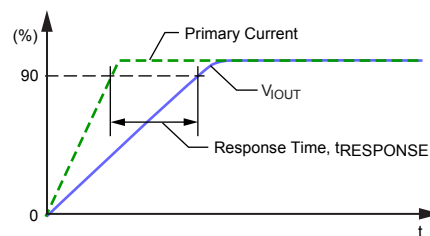
Figure 8: Response Time ( t_{\text{RESPONSE}} )
