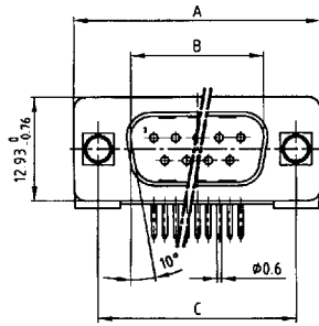
Plug connector
