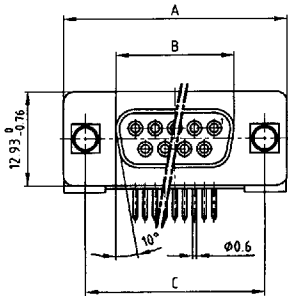
Socket connector
