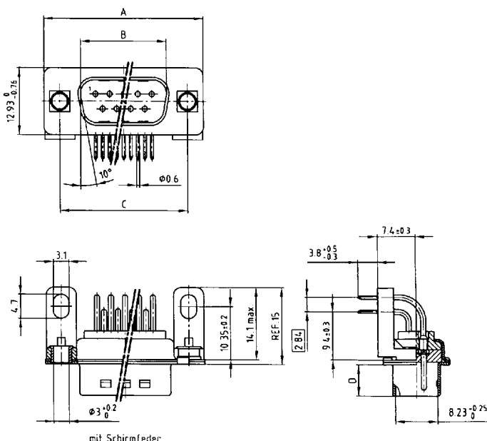
Plug connector
