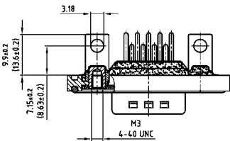
Mounting style: PCB clip, threaded insert
