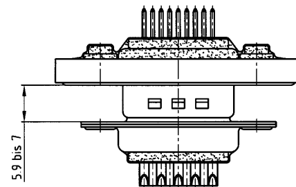
Rigid mount vertical to tolerance guide
