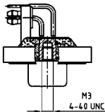
Mounting style: PCB clip, threaded insert
