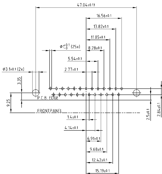
PCB layout Kat1kGSA (View: component side)
