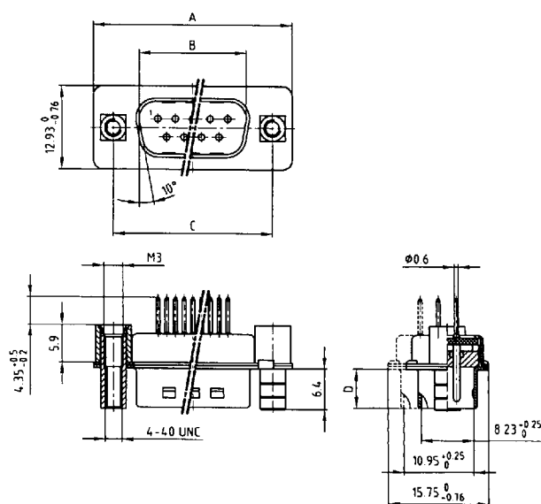
Plug connector
