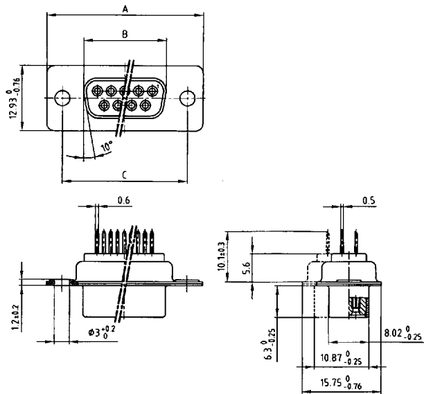
Socket connector
