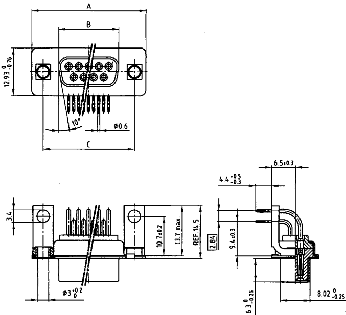
Socket connector
